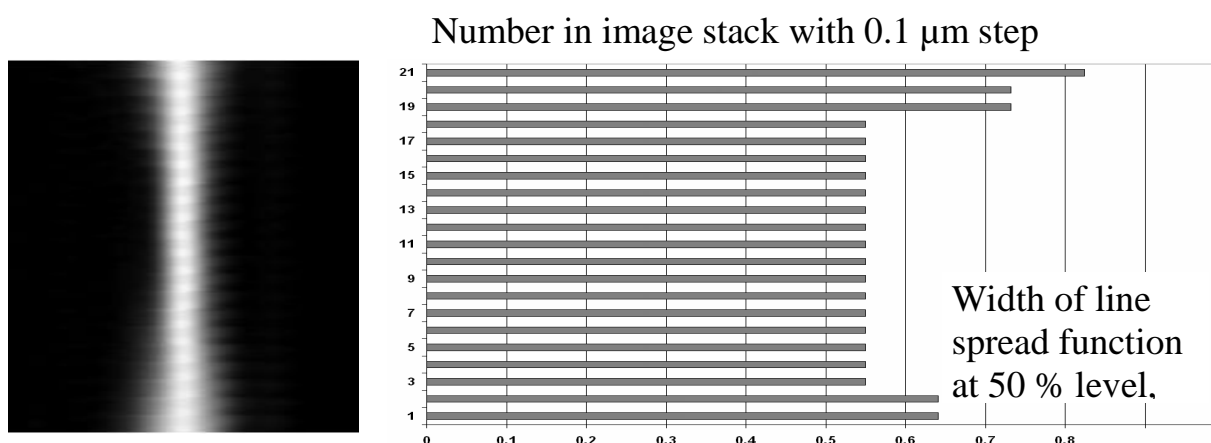
Fig. 1. Focus diagram and the width of line spread function at 50 % level as a function of defocusing.
